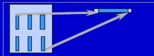
(b) Regular series of blocks from a 2D array to a contiguous sequence at a certain offset in a 1D array
