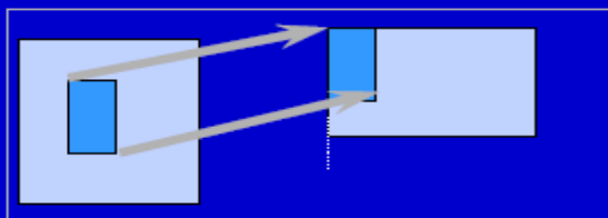
(a) Hyperslab from a 2D array to the corner of a smaller 2D array
