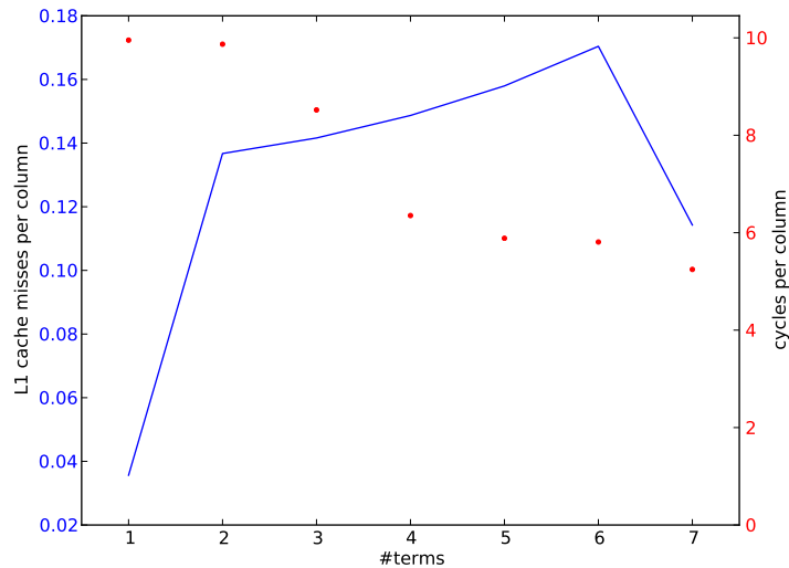
Figure 1.21: The number of L1 cache misses and the number of cycles for each j column accumulation, vector length 4096 + 8
