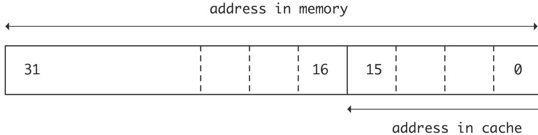
Figure 1.8: Direct mapping of 32-bit addresses into a 64K cache
