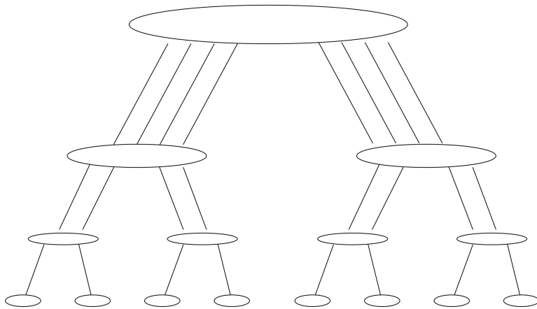
Figure 2.27: A fat tree with a three-level interconnect (left); the leaf switches in a cabinet of the Stampede cluster (right)
