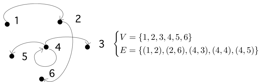
Figure 20.1: A simple graph
