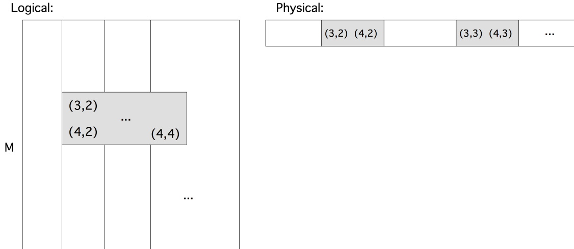
Figure 29.2: A subblock out of a larger matrix
