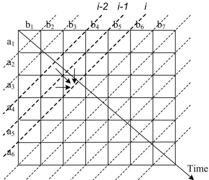
Figure 12.1: Illustration of dependencies in the Smith-Waterman algorithm; diagonals are seen to be independent
