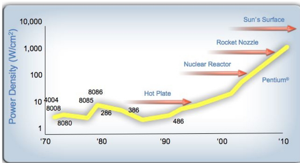
Figure 1.28: Projected heat dissipation of a CPU if trends had continued – this graph courtesy Pat Helsing. The illustration shows the heat that a chip would give off, if single-processor trends had continued.
