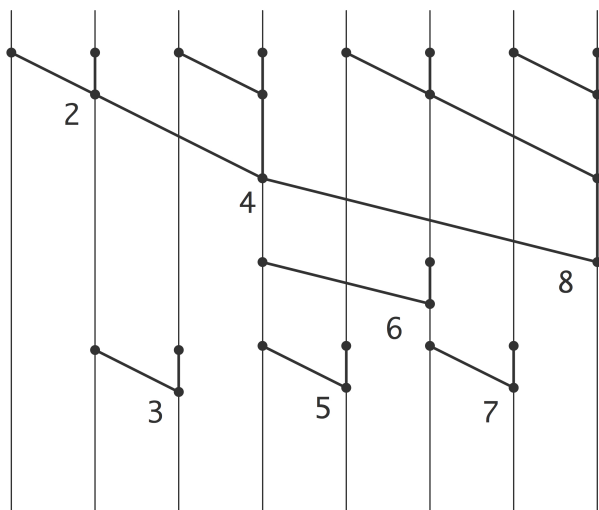
Figure 23.1: A prefix operation applied to 8 elements
