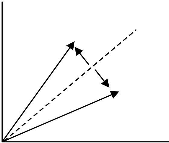
Figure 16.1: Householder reflector
