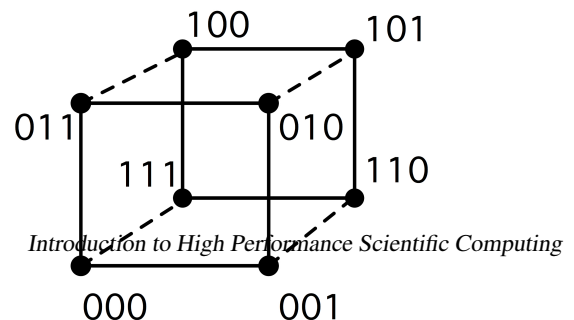
Figure 2.22: Gray code numbering of the nodes of a hypercube
