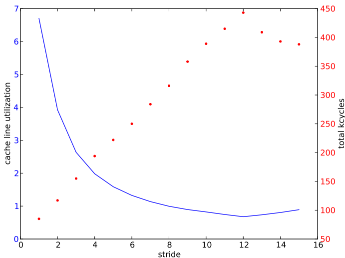
Figure 37.1: Run time in cycles and L1 reuse as a function of stride
