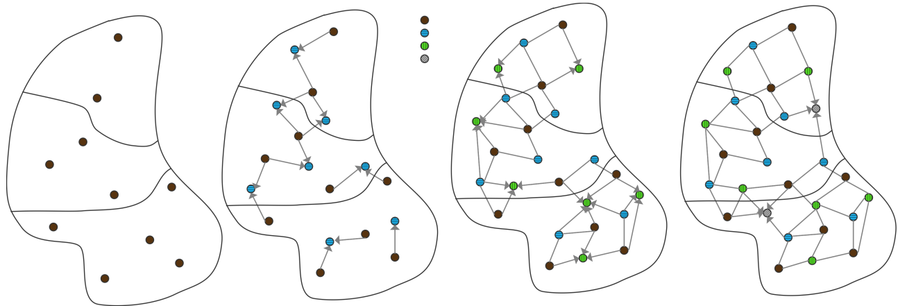
Figure 6.12: Solving a parallel multicolour ILU in four steps
