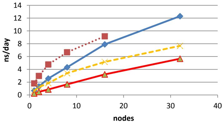
NAMD 2.10 Xeon PHI performance (Galileo)
