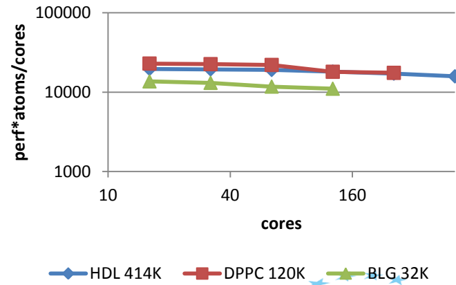
Gromacs weak scaling
