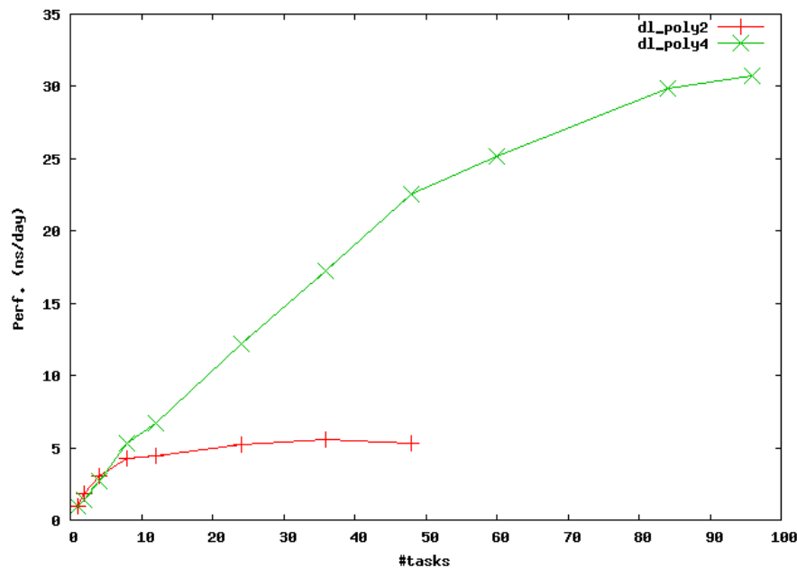
Comparison of DL_POLY(Classic) and DL_POLY 4.x
